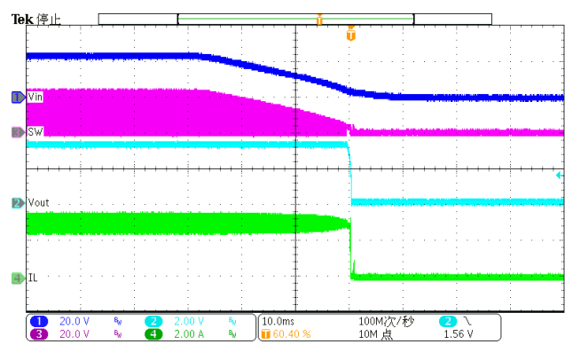
Figure 13. Power down(Iload=3A)
